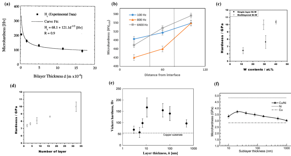
Fig. 37. Vickers microhardness of (a) Ni-30%Sn multilayer coatings in accordance with thickness of layers (d) [159] and (b) Ni-Fe-Al 2 O 3 gradient coatings at different distances under the sublayer [36,199]. the effect of (c) tungsten content and (d) number of bilayers on the hardness of Ni-W multilayer coatings [27]. hardness of (e) Ni/Cu nano-scaled multilayer coatings versus thickness of layers [93], (f) Cu/Ni multilayer and copper and nickel monolithic coatings Hardness versus thickness of the sublayer [83].
