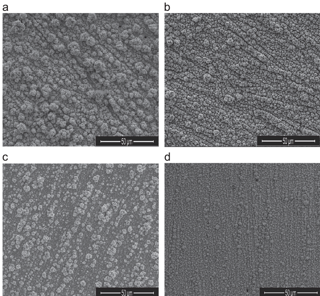
Fig. 15. Effect of increasing copper thickness on Co-Fe/Cu multilayer structure at a Cu thickness of (a) 0 nm, (b) 3 nm, (c) 4.5 nm and (d) 6 nm [75].
