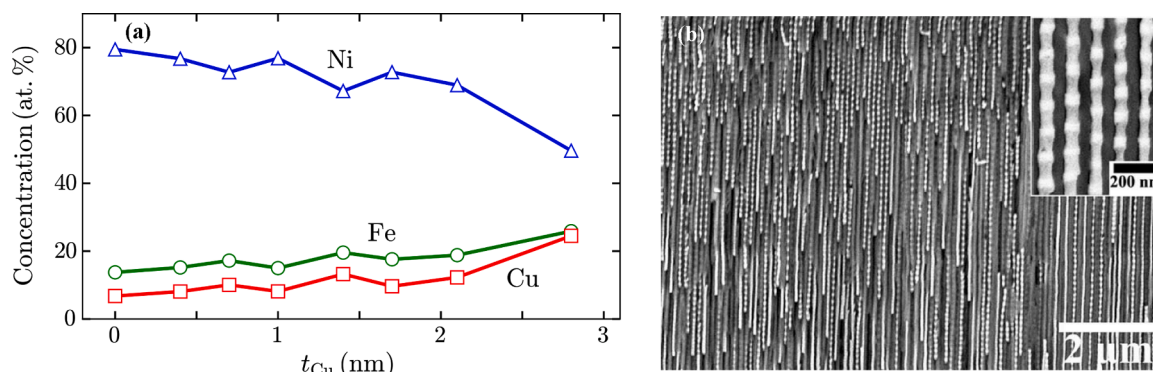
Fig. 18. (a) The effect of copper layer thickness t_{Cu} on the concentration of alloying elements in Fe-Ni-Cu/Cu multilayer [120]. (b) SEM image of bamboo-like structure of Co/Pt multilayer [136].
