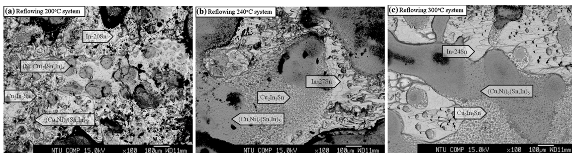
Fig. 23. Fracture surface of the Cu/Sn/(In/Ni/Cu/Ni/In)/Sn/Cu sandwich multilayer coating after the shear test at (a) 200 °C, (b) 240 °C and (c) 300 °C [168].
