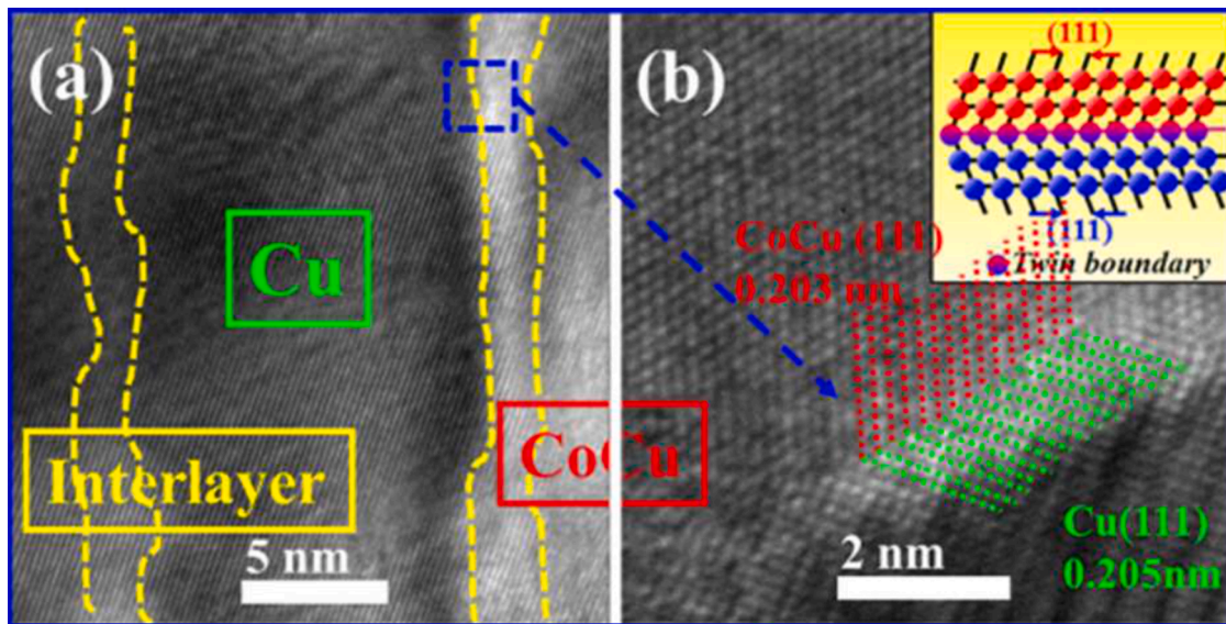
Fig. 16. TEM image of a Cu/Co 81 Cu 19 multilayer, (a) the multilayer and the zig-zag interface between layers, (b) the accumulation of layers on each other and twinning [73].
