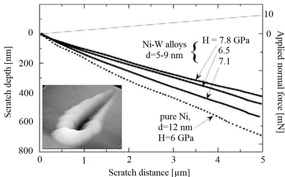
Fig. 33. Scratch depth diagrams based on the position of the diamond cone peak moving over the sample surface. The second traverse axis shows the normal load of the diamond peak. In addition, AFM micrograph illustrates a scratch surrounded by a mass bulk of material. The scratch length in this micrograph is 5 μm [206].
